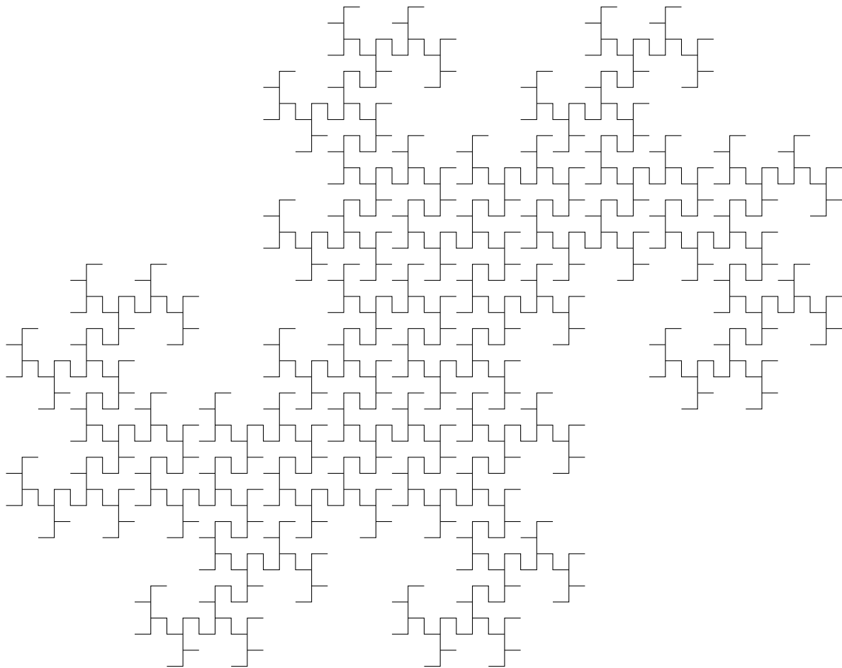
Twindragon area tree level 10, after Mandebrot
