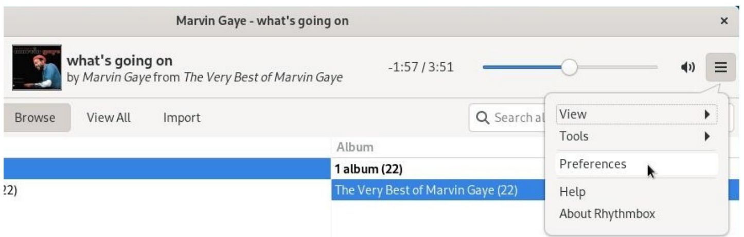
Rhythmbox: menu
