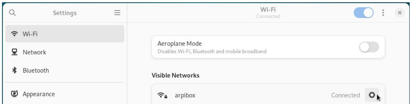
Network selection
