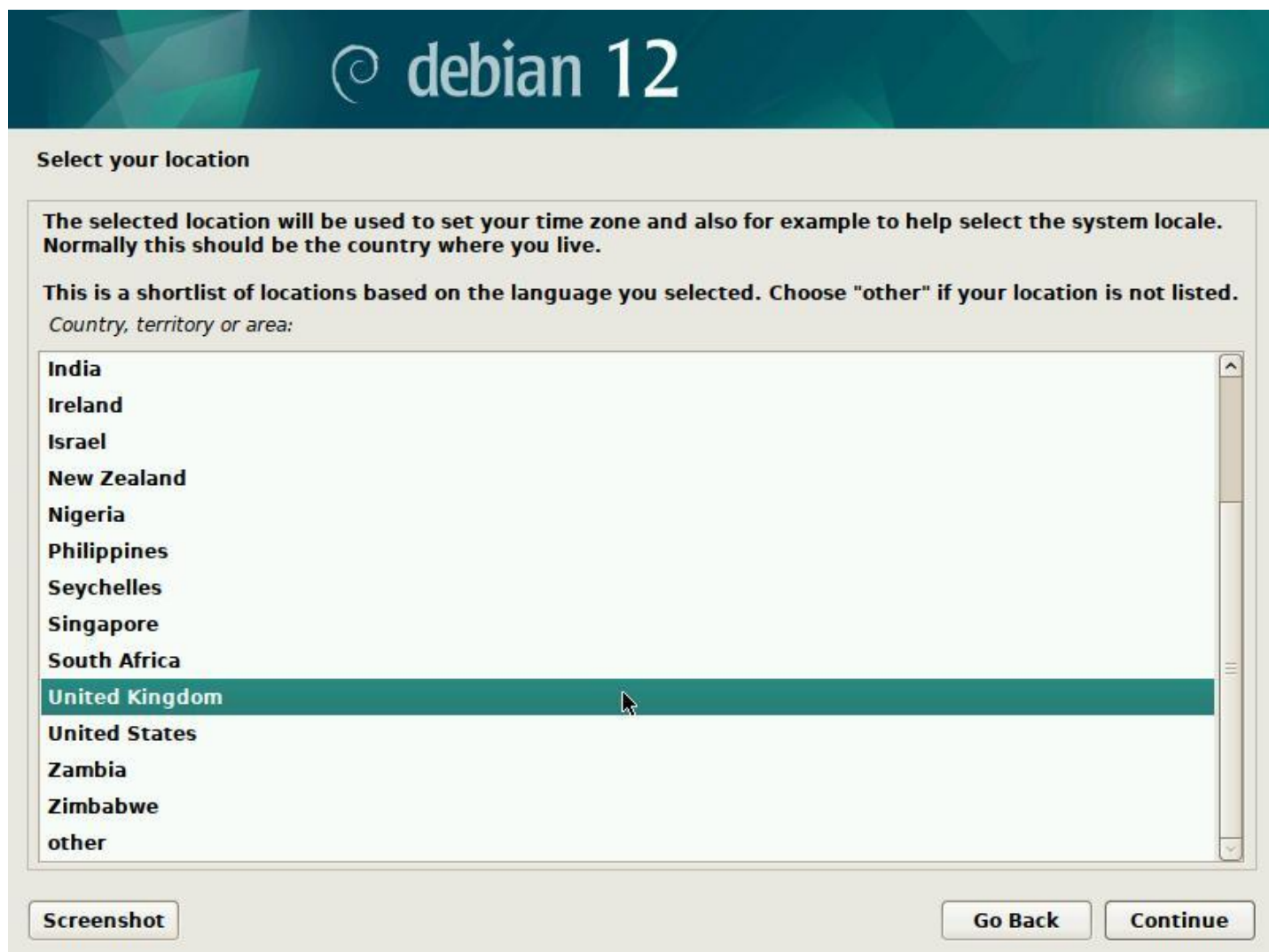
Installation: country
