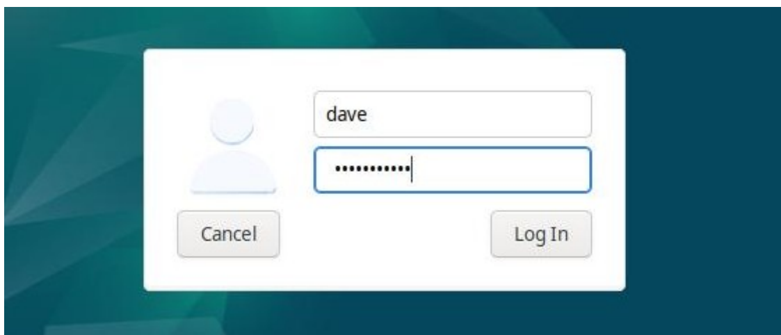
LightDM
