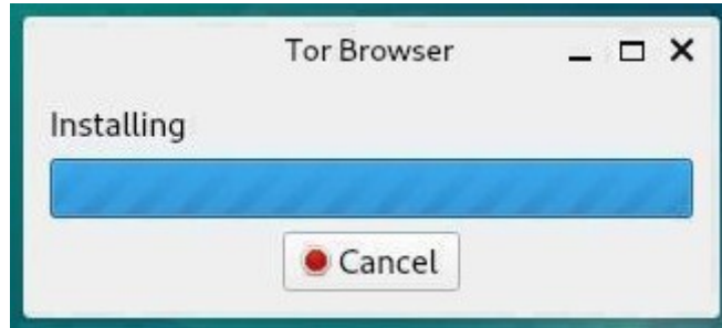
TorBrowser: installing
