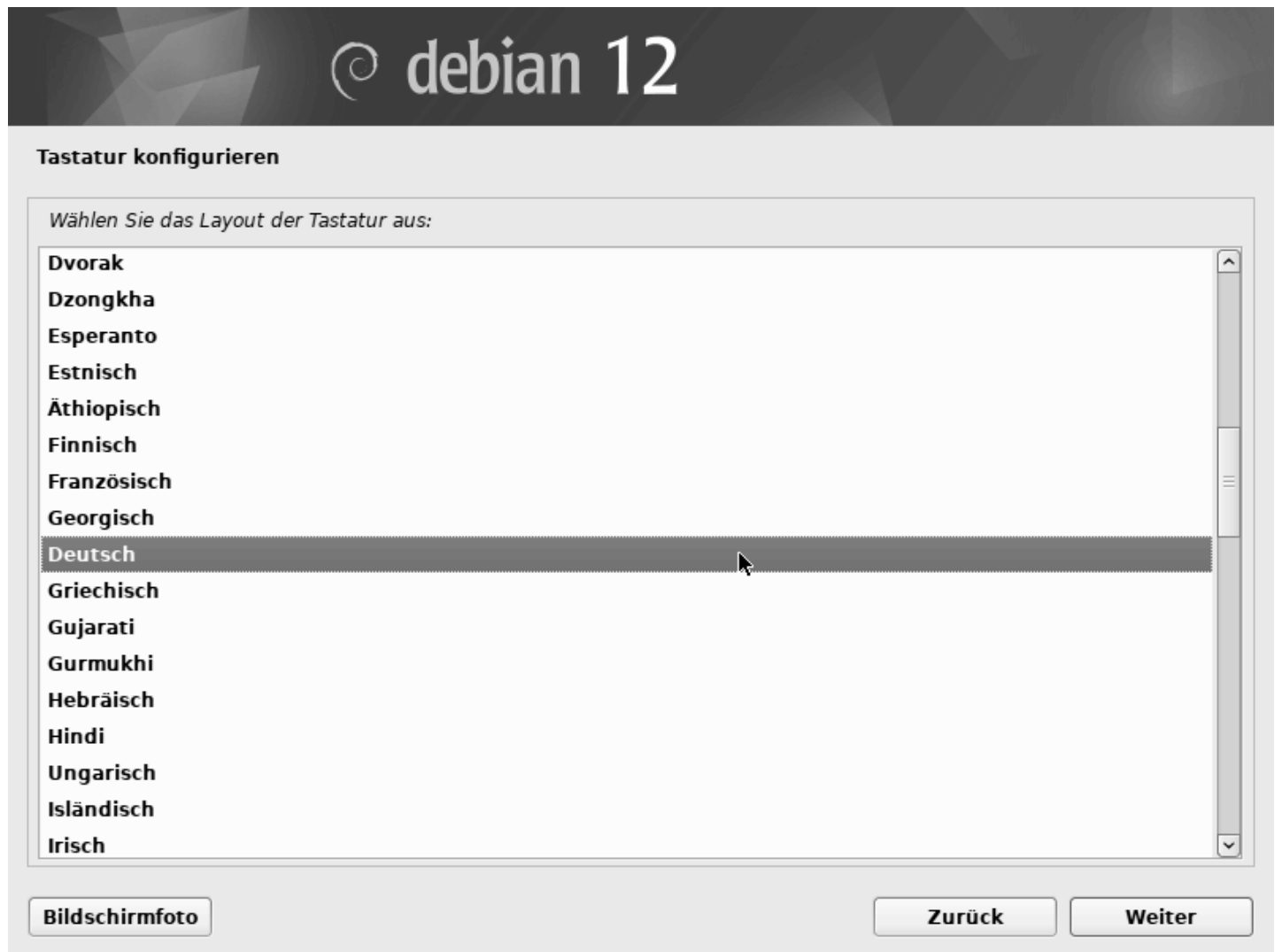
Installation: Tastatur
