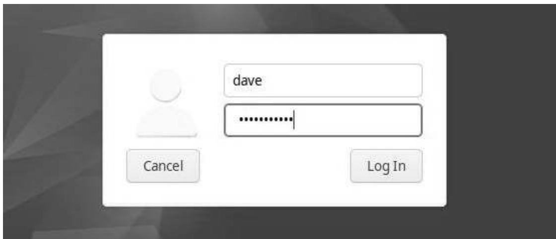
LightDM
